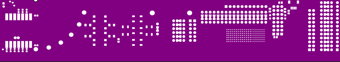
Top Solder (Scale 1:1.43)
